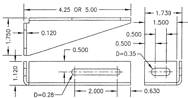
3 HURRICANE BRACKET
