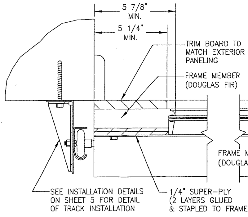
SECTION D SCALE: 1/4 FULL
