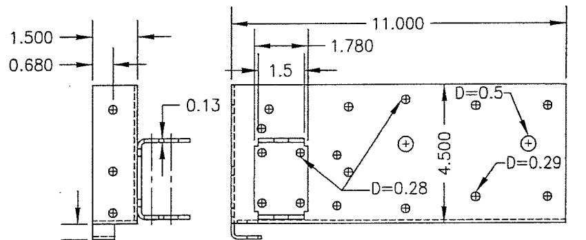
SLIDE LOCK DETAIL (MAY BE LOCATED AT EITHER SIDE OF DOOR)
