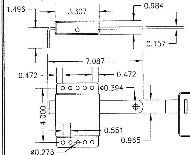
22 SLIDE LOCK
