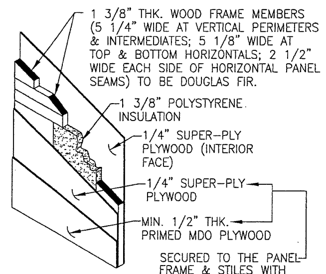
TYP. FLAT PANEL
