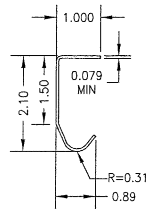
9 TRACK
