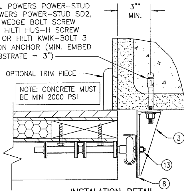
INSTALLATION DETAIL DIRECT TO FILLED BLOCK OR SOLID CONCRETE
