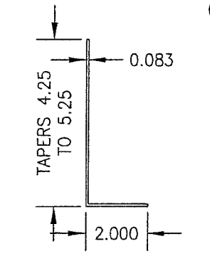
8 TRACK ANGLE
