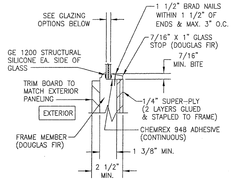
GLAZING DETAIL
