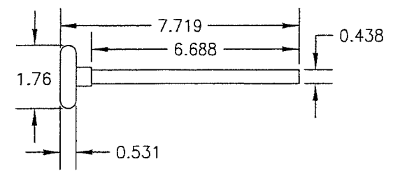
1 NYLON ROLLER WITH AISI STEEL ROD
